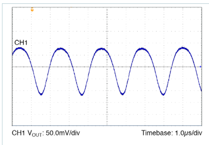
Figure 46 — Output Voltage Ripple: Nominal Line, Nominal Trim, 100% load, C_{OUT} = 8 \times 10\mu F Ceramic
