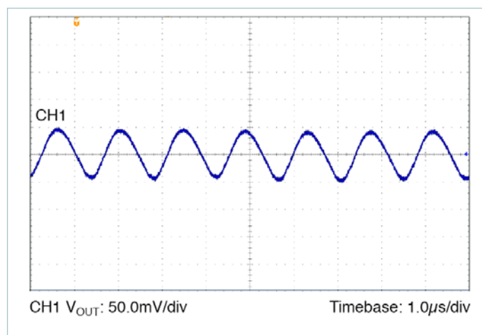
Figure 49 — Output Voltage Ripple: Nominal Line, Nominal Trim, 50% load, C_{OUT} = 8 \times 10\mu F Ceramic
