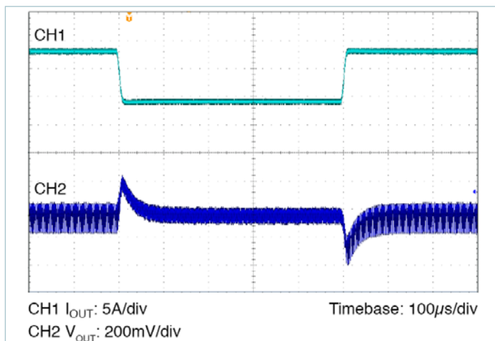
Figure 45 — Transient Response: 50% to 100% load, at 1A/μs. Nominal Line, Nominal Trim, C_{OUT} = 8 \times 10\mu F Ceramic
