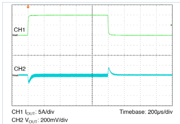
Figure 19 — Transient Response: 50% to 100% load, at 1A/μs. Nominal Line, Nominal Trim, C_{OUT} = 12 \times 47\mu F Ceramic
