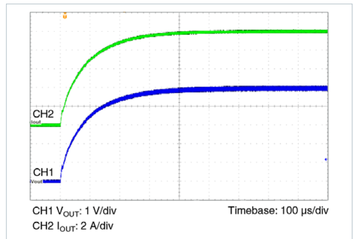
Figure 16 — Start Up, C_{REF} = 0 ( V_{IN} = 28\text{ V} , I_{OUT} = 10\text{ A} , C_R , C_{OUT} = 6 \times 10\text{ }\mu\text{F X7R Ceramic} )
