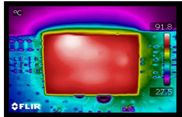
Figure 20 — Thermal Image ( V_{IN} = 28 V, I_{OUT} = 10 A, CR, 0 LFM Evaluation PCB)
