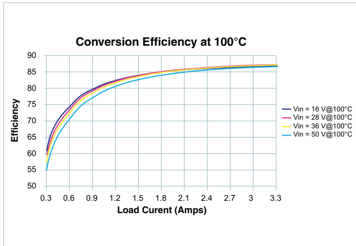
Figure 31 — Conversion Efficiency
