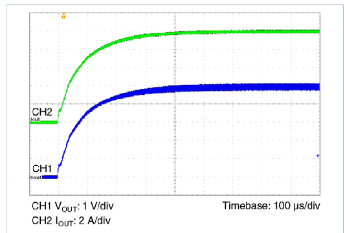
Figure 15 — Start Up, C_{REF} = 0 ( V_{IN} = 16\text{ V} , I_{OUT} = 10\text{ A} , C_R , C_{OUT} = 6 \times 10\text{ }\mu\text{F X7R Ceramic} )
