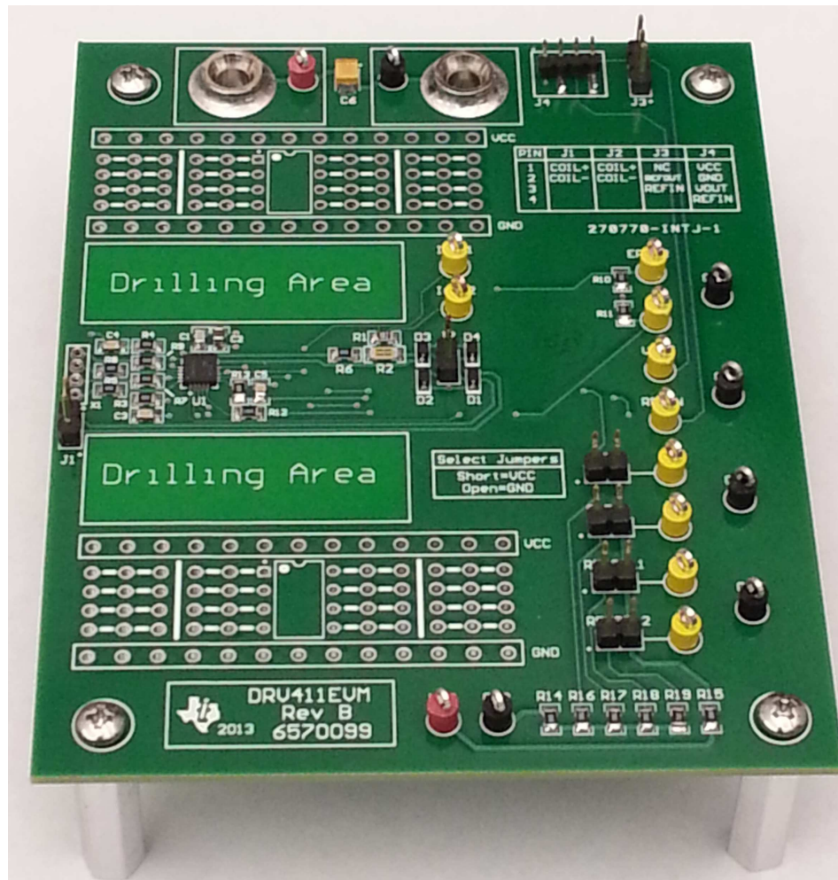
Figure 1. DRV411EVM Board
