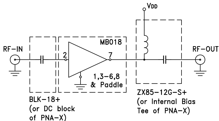
Fig 1. Characterization Circuit
