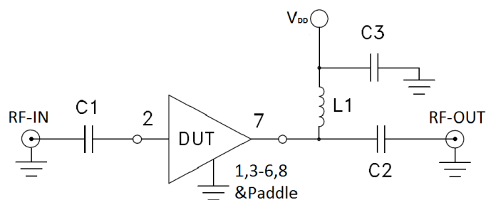
Fig 2. Application Circuit
