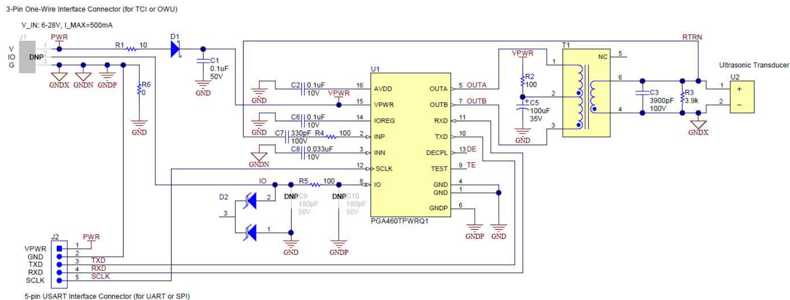
Figure 6. PGA460PSM-EVM Schematic
