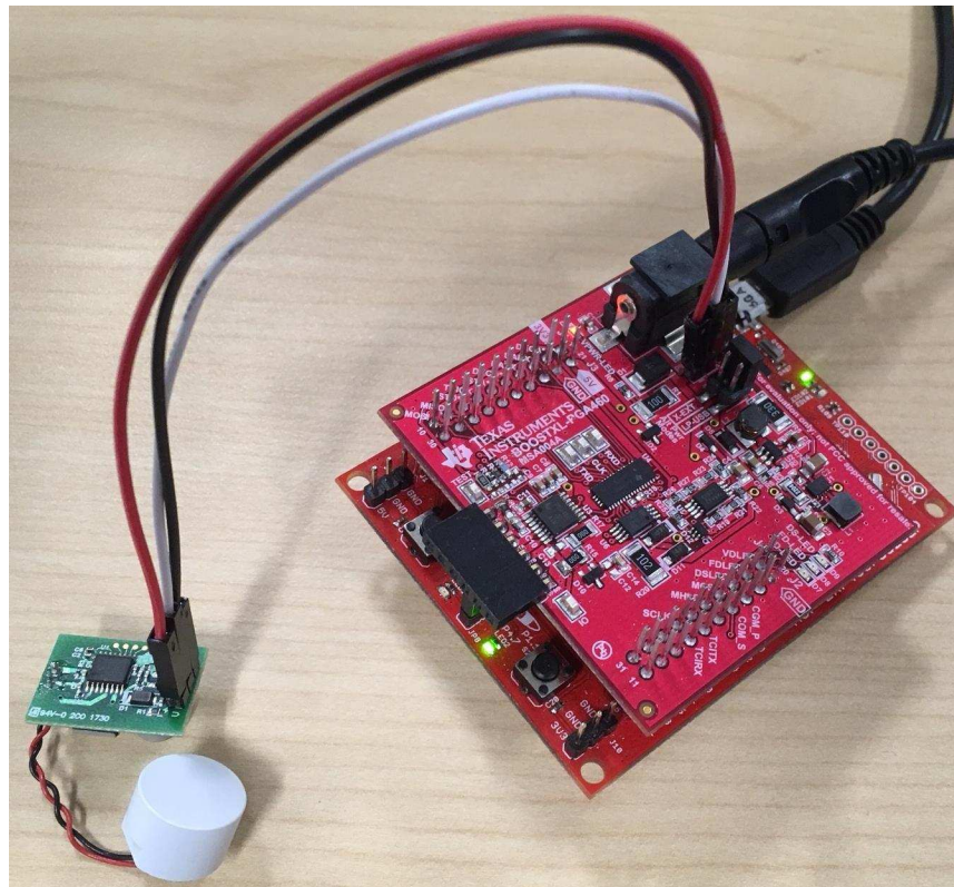
Figure 3. External OWI Evaluation Setup for PGA460PSM-EVM With Software Modification
