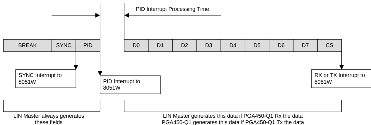
Figure 34. LIN Interrupts
