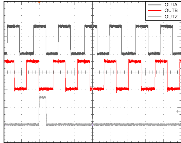
OUT A,B,Z during a constant velocity rotation
