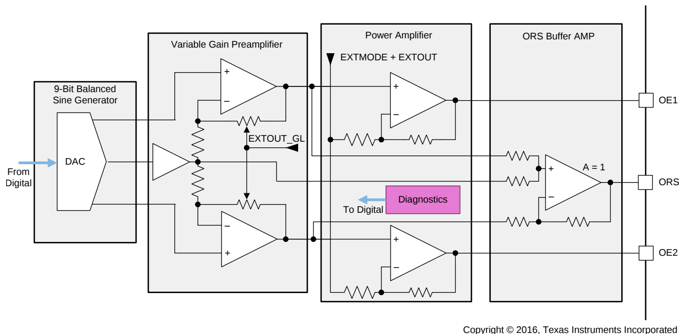
Figure 12. Exciter Signal Generation Circuit
