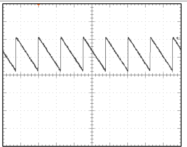
Figure 76. AOUT Signal (With No Resolver Connected)
