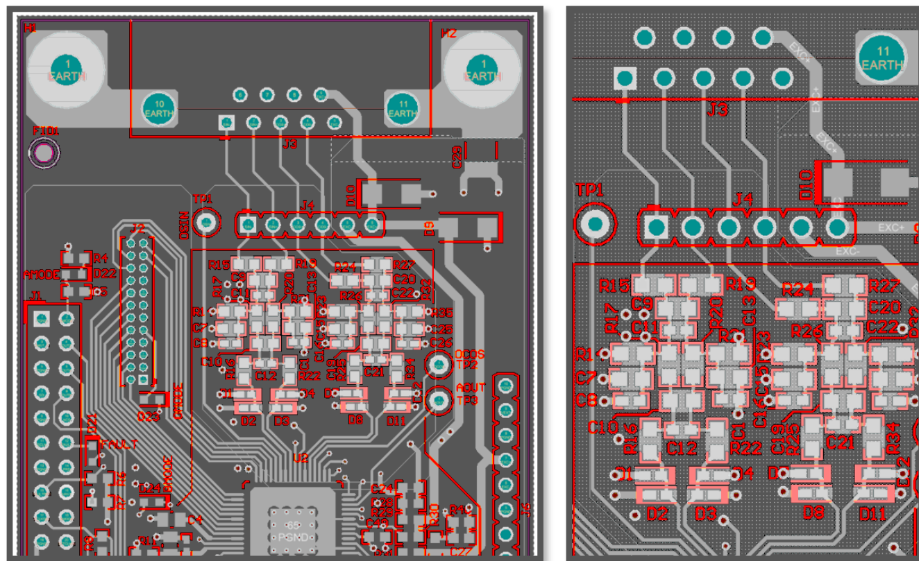
Figure 86. Analog Front-End Layout
