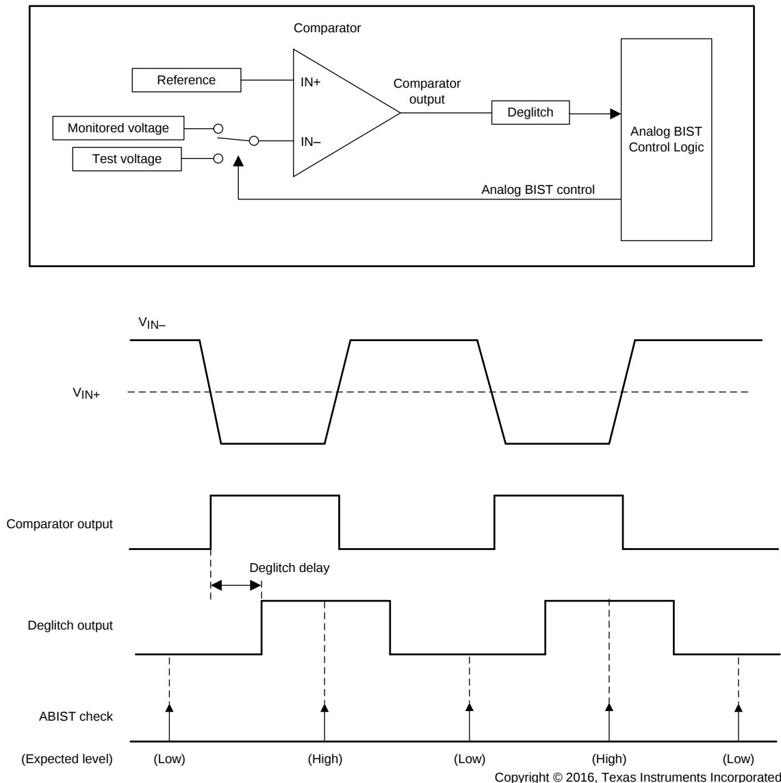
Figure 39. BIST
