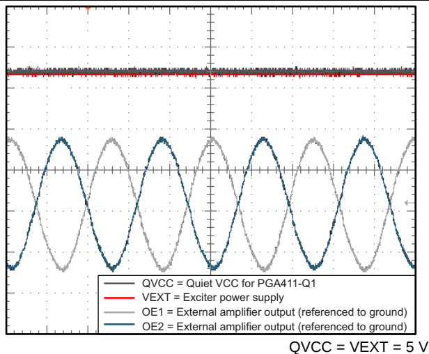
Figure 74. Exciter Amplifier
