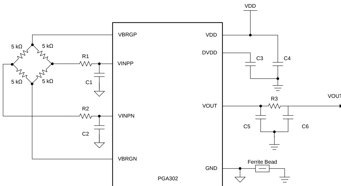
Figure 116. Application Schematic
