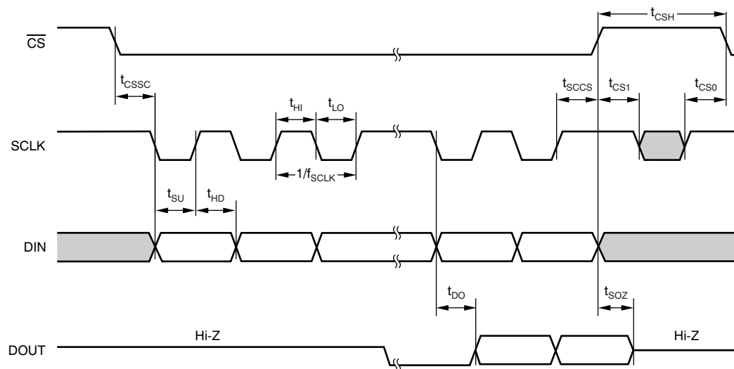
Figure 2. SPI Mode 1, 1
