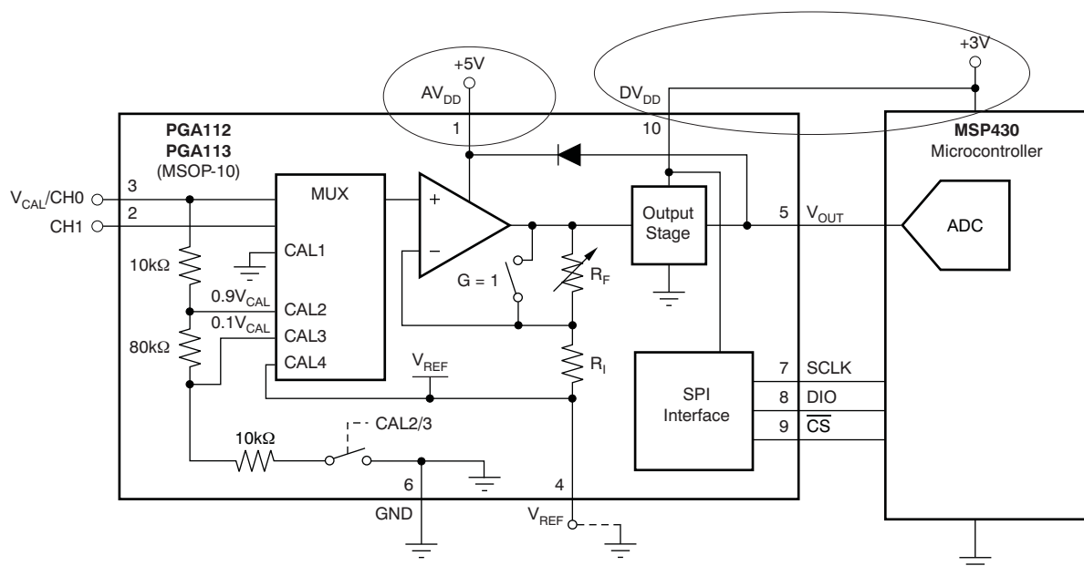
Figure 76. Split Power-Supply Architecture: AV_{DD} \neq DV_{DD}
