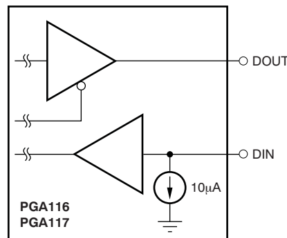
Figure 57. Digital I/O Structure—PGA116 and PGA117
