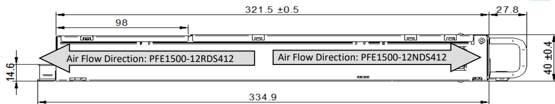
Figure 24. Side View 1
