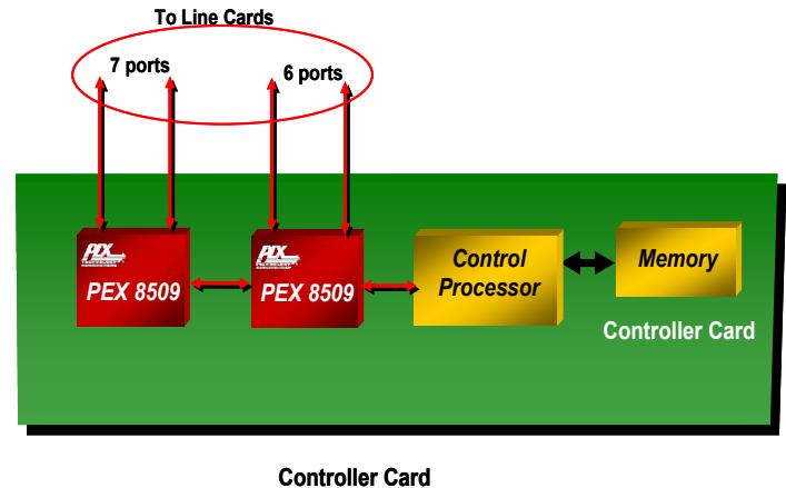
Figure 5. Control Plane for Large Systems
