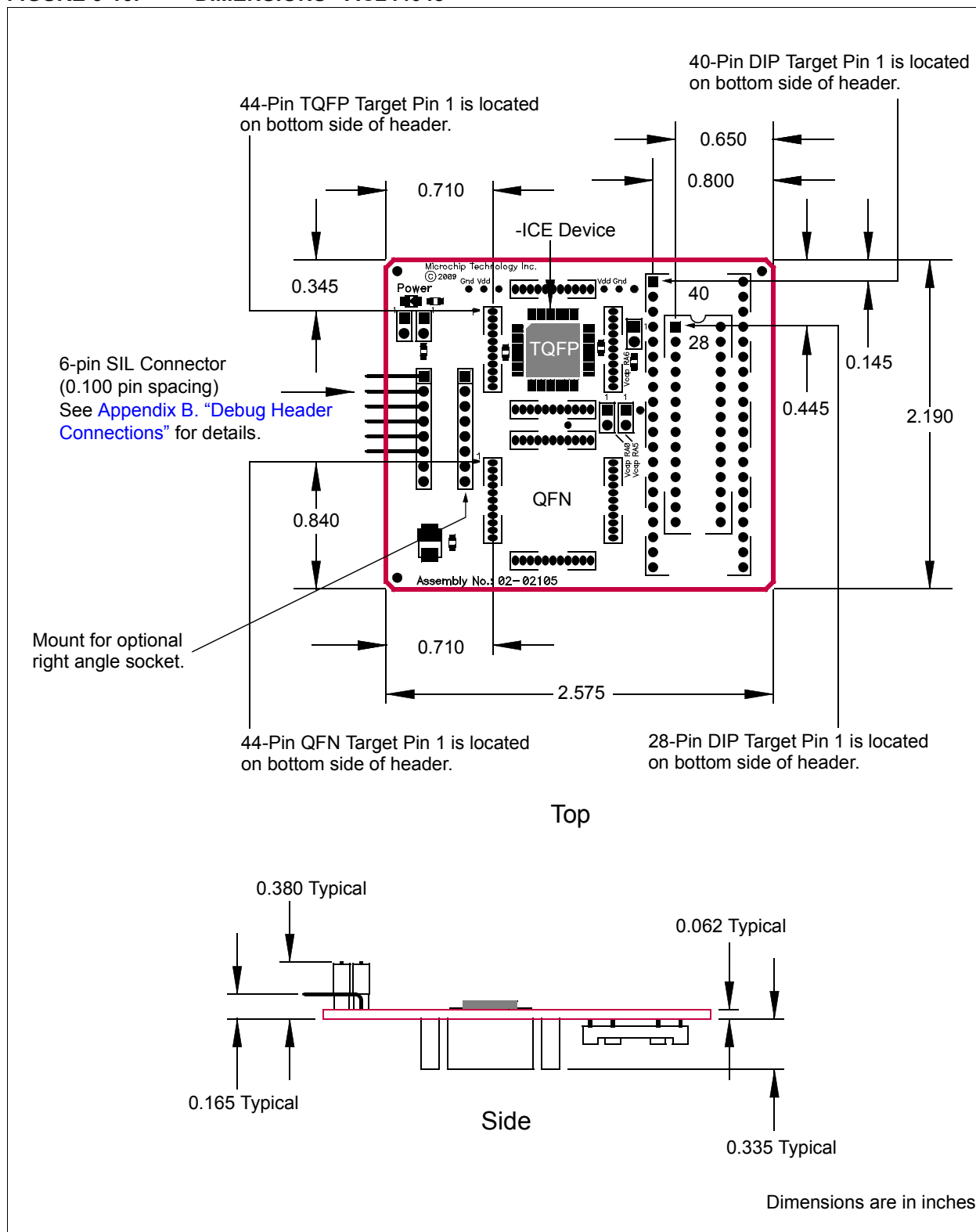
FIGURE 3-16: DIMENSIONS - AC244048
