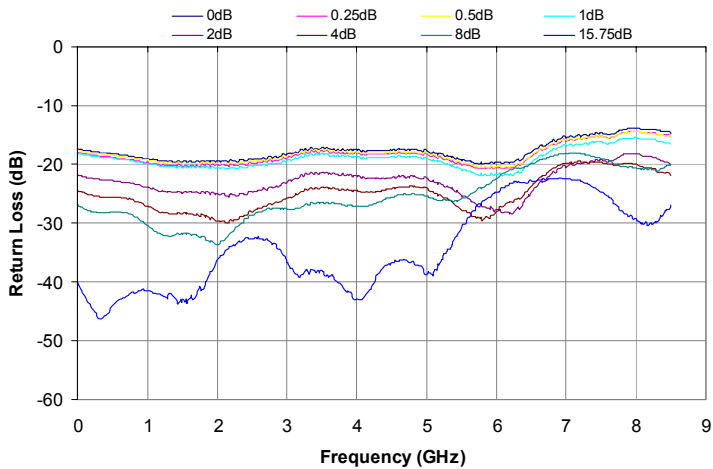
Figure 9. Output Return Loss vs. Attenuation: T = +25C
