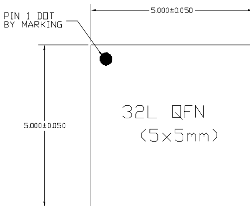
Figure 24. Package Drawing
