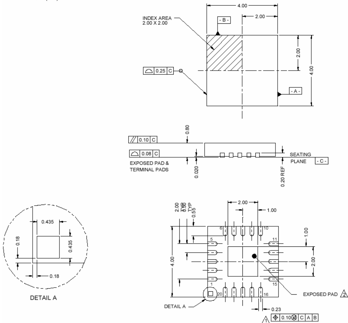
Figure 16. Package Drawing
