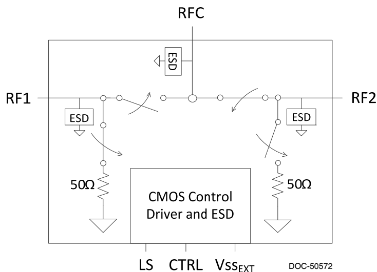
Figure 1. Functional Diagram
