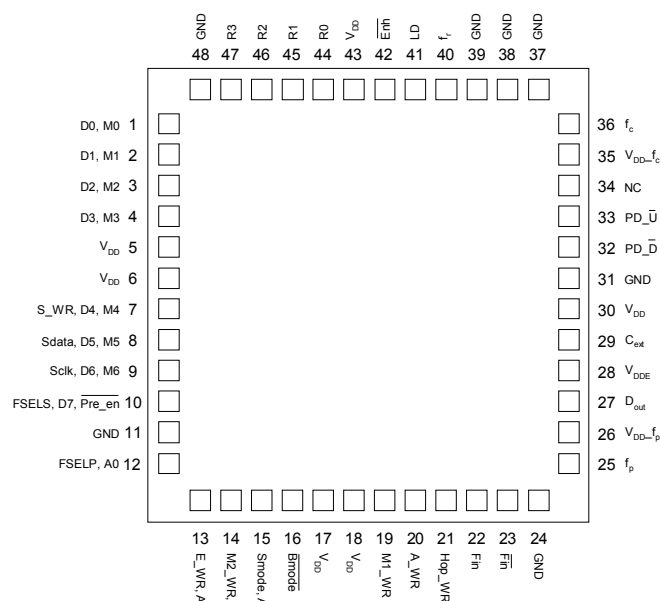
48-lead QFN
