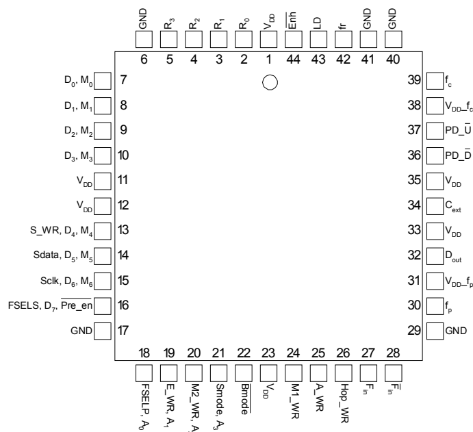
44-lead PLCC
