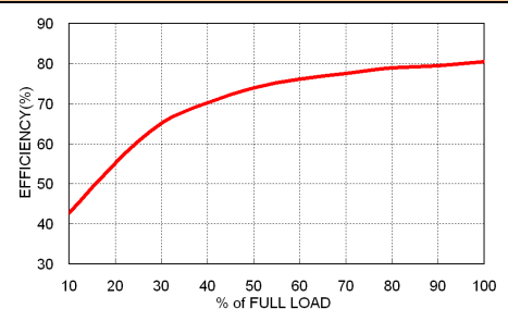
PDS02-48S05 Efficiency vs. Output Load
