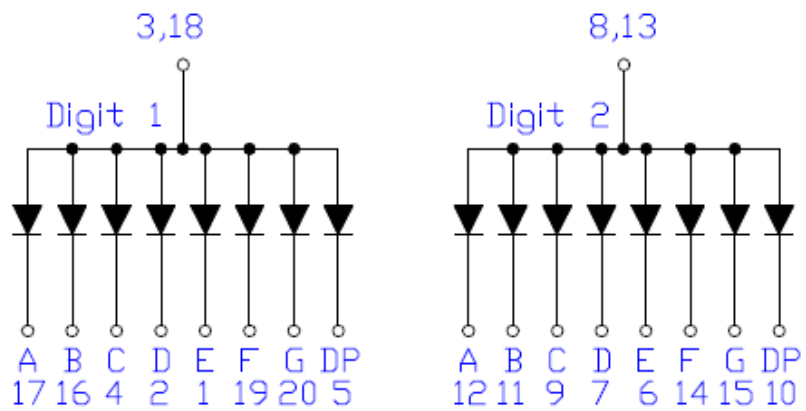
Common Anode
