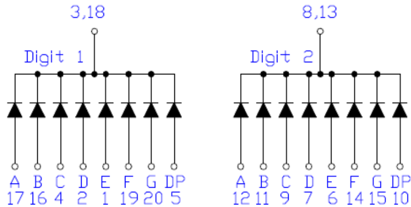
Common Cathode
