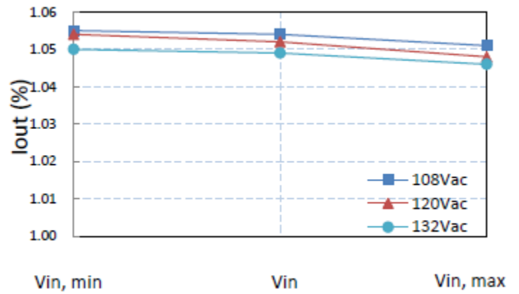
Load (Vout) &amp; Line (Vin) regulation
