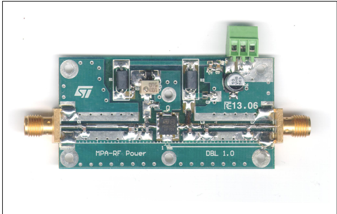
Figure 14. Demoboard photo
