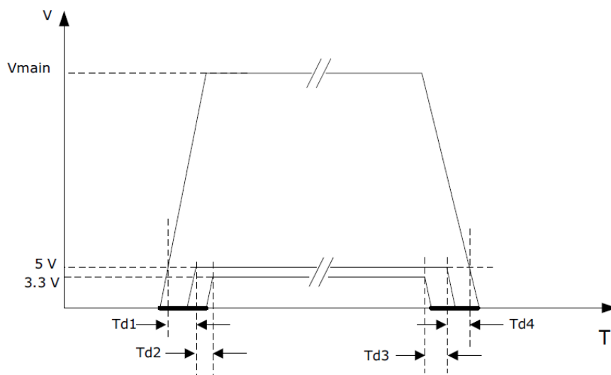
Figure 4-2. Power Sequencing
