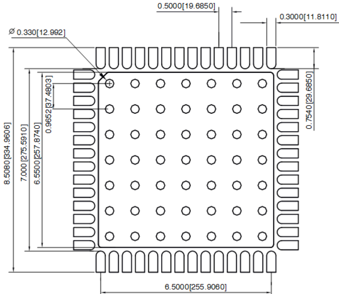
Figure 5-2. Top-Copper Layer
