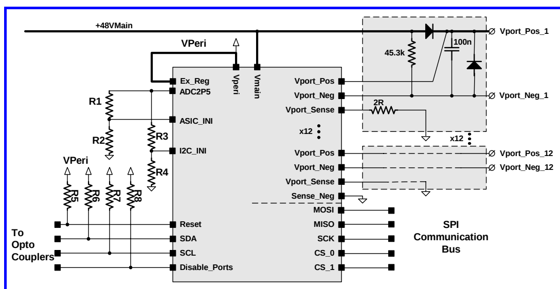
Figure 7 - Single-port Application with AC Disconnect Support
