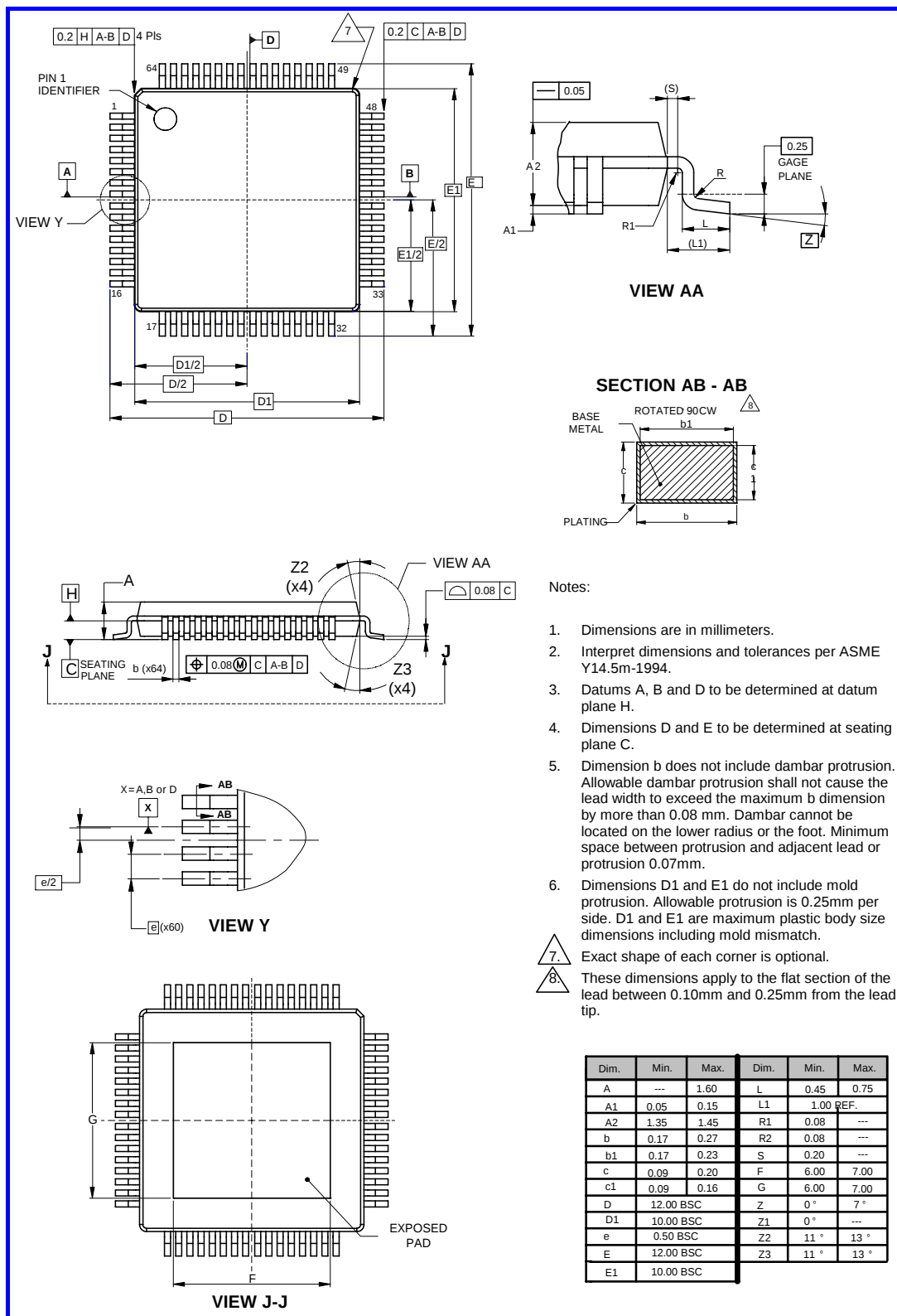
Figure 6: PD64012 Mechanical Dimensions
