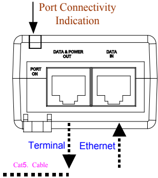
Figure 1: Connecting the PD-3501G
