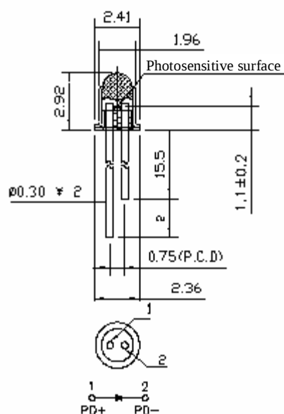
PD-1153-XXX (Dome Lens Cap)
