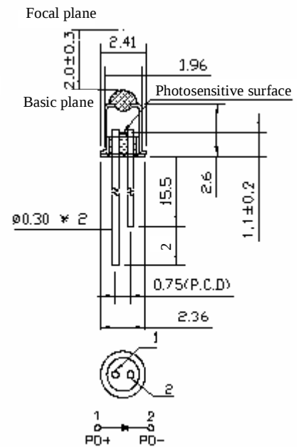
PD-1155-XXX (Ball Lens Cap)
