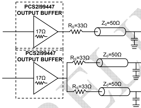
Figure 2. Single versus Dual Transmission Lines
