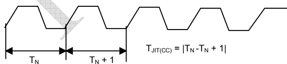
Figure 9. Output Duty Cycle (DC)
