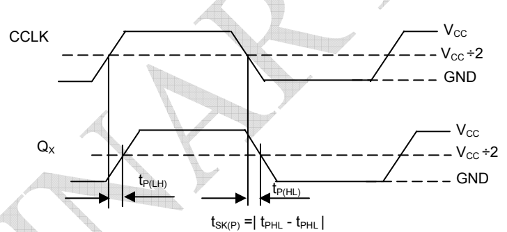
Figure 8. Output Pulse Skew ( t_{SK(P)} ) Test
