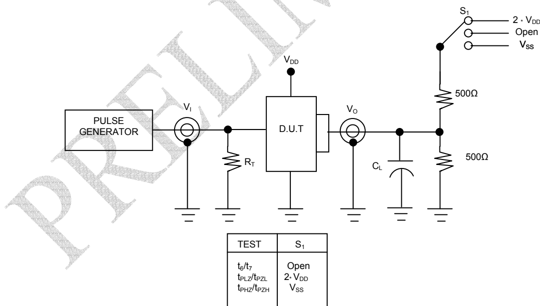
Figure 1. Load circuit for Switching times
