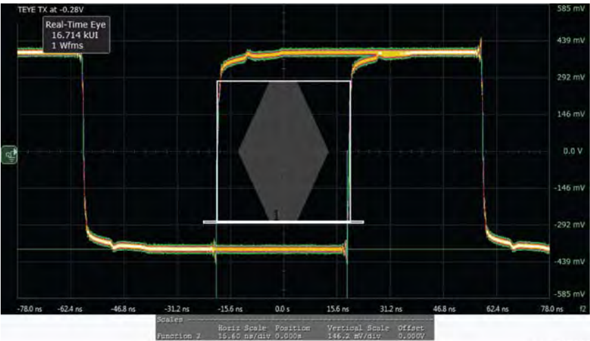
Fig 15. MIPI M-PHY PWM-TX transmitter eye opening at –140 mV, test board with PCMF2USB3S; typical values
