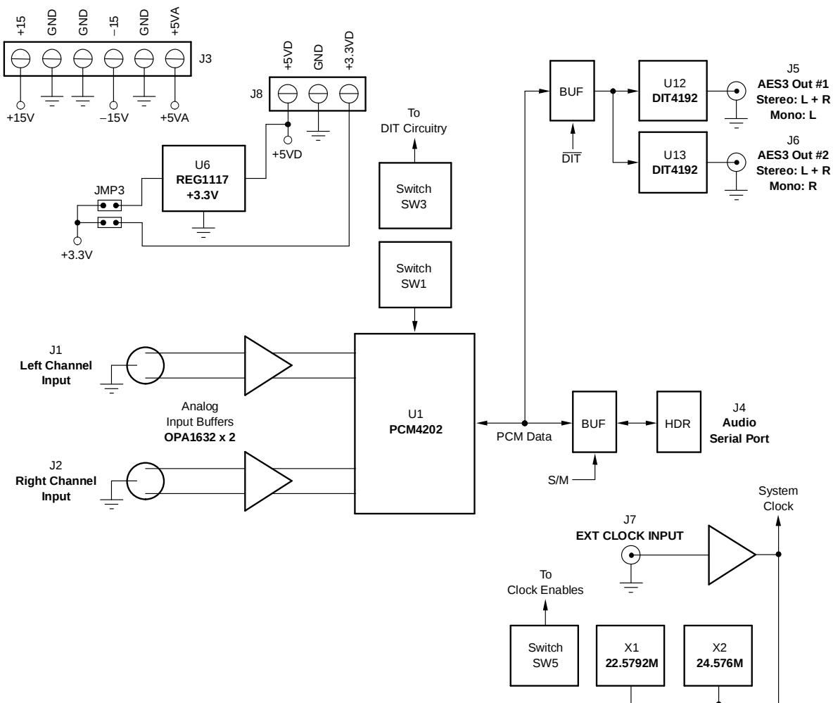
Figure 2. PCM4202EVM Functional Block Diagram
