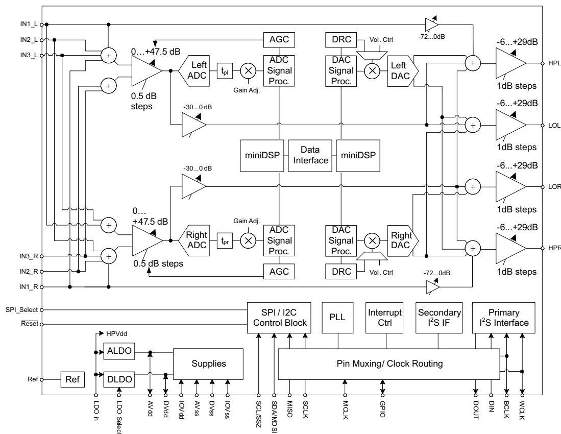
Figure 18. Block Diagram
