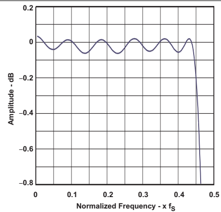
Figure 10. Passband Ripple
