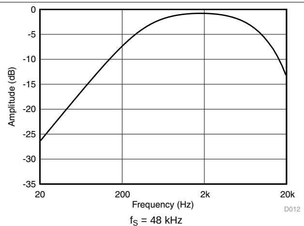
Figure 17. Secondary ADC Frequency Response
