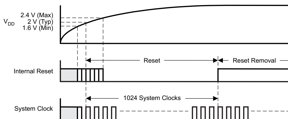
Figure 33. Power-On-Reset Timing
