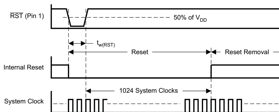
Figure 33. Power-On-Reset Timing
