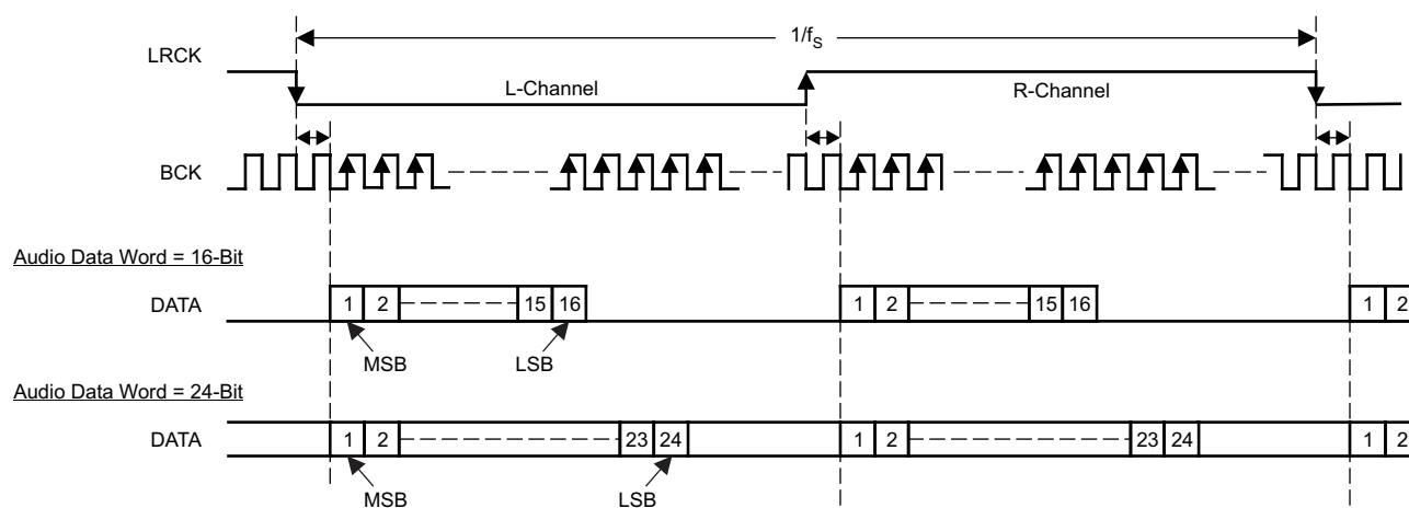
Figure 35. Audio Data Input Formats
