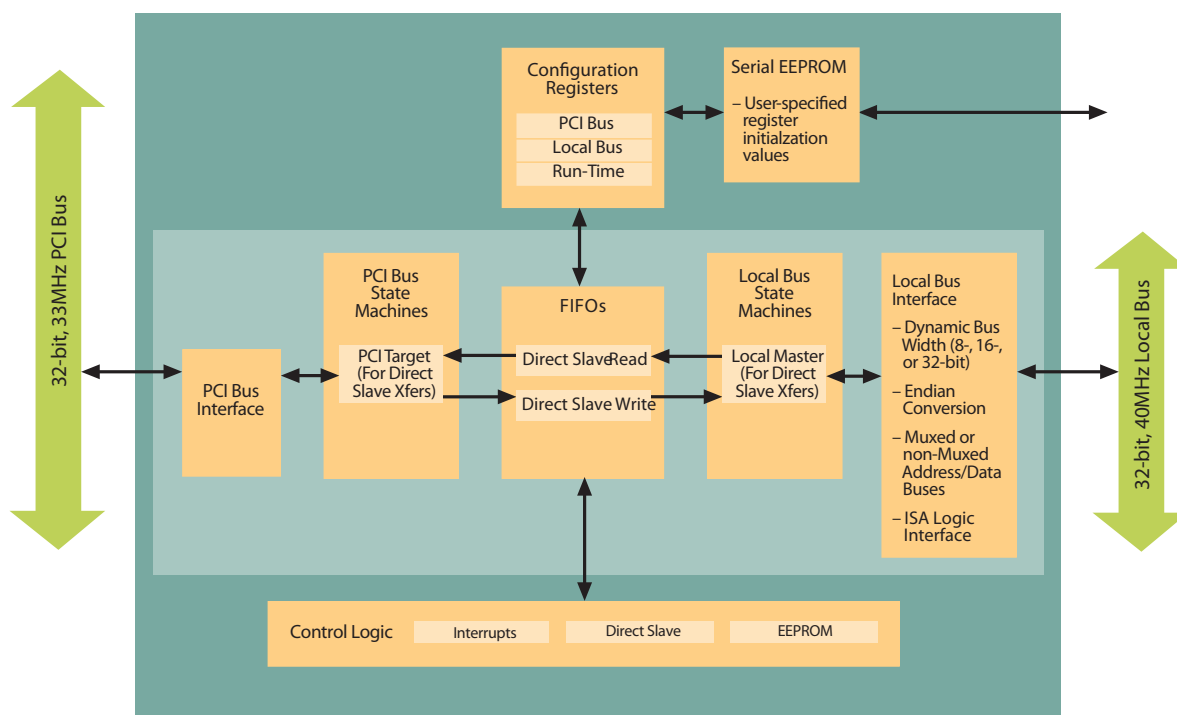
PCI 9052 Internal Block Diagram
