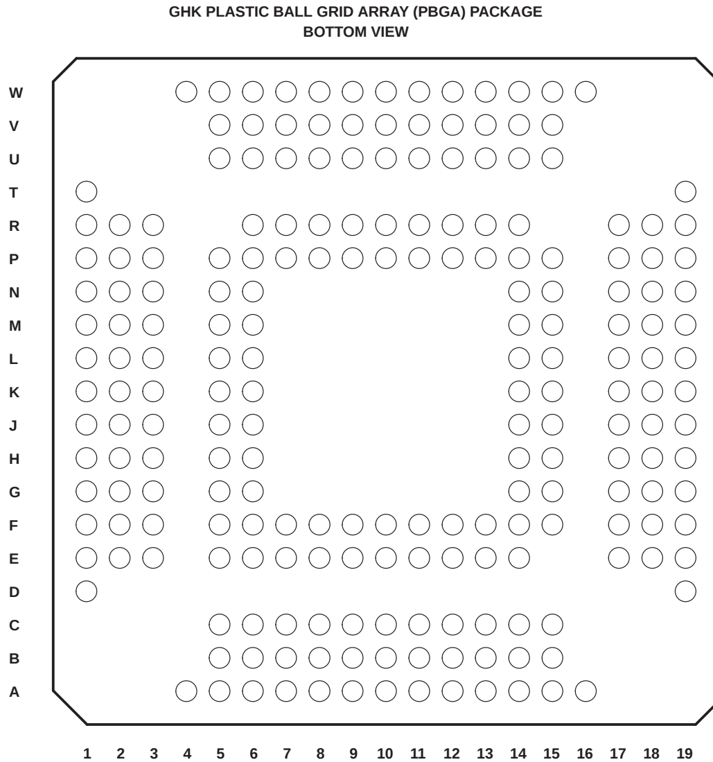
Figure 2–1. PCI1520 GHK-Package Terminal Diagram
