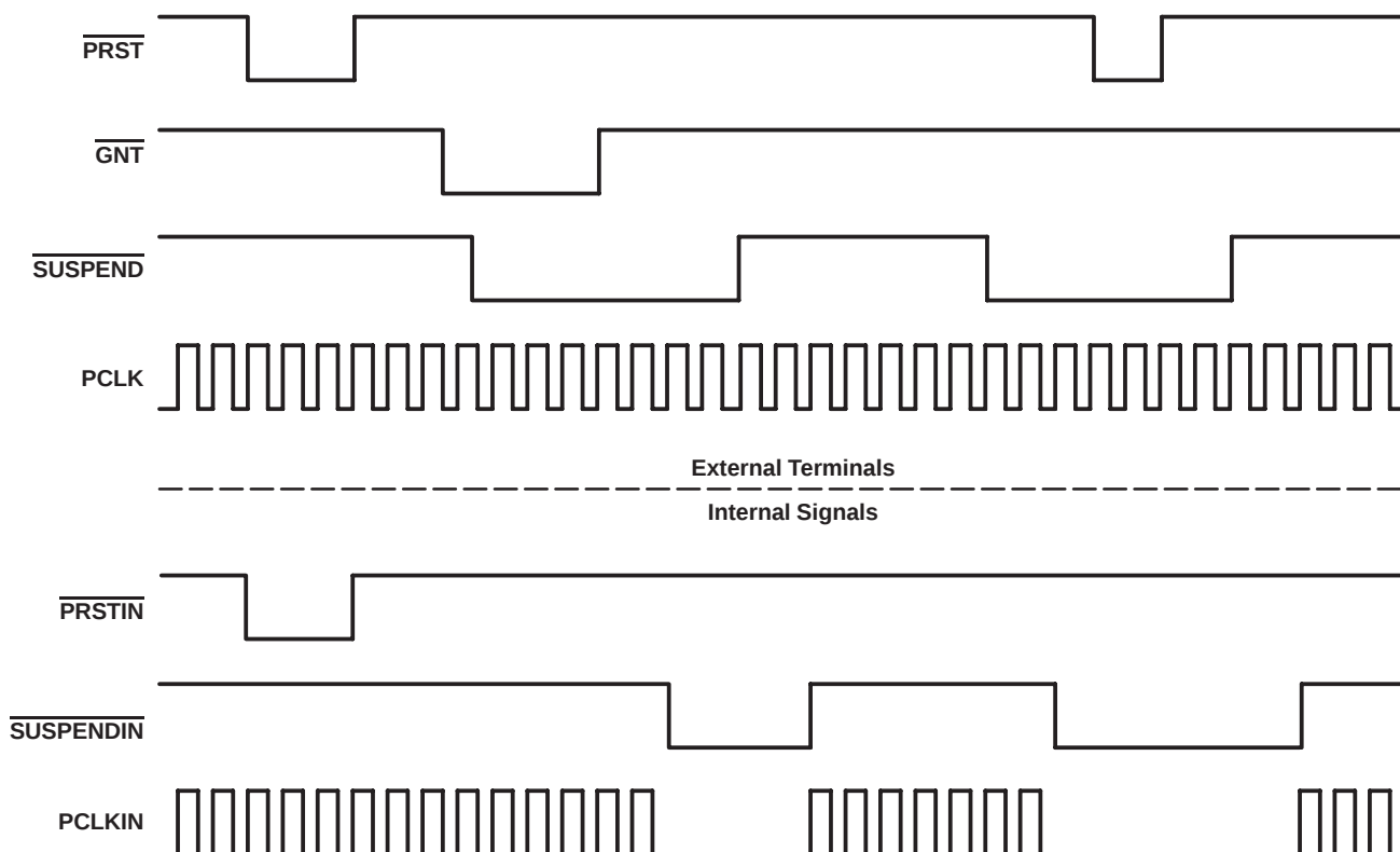
Figure 18. Signal Diagram of Suspend Function
