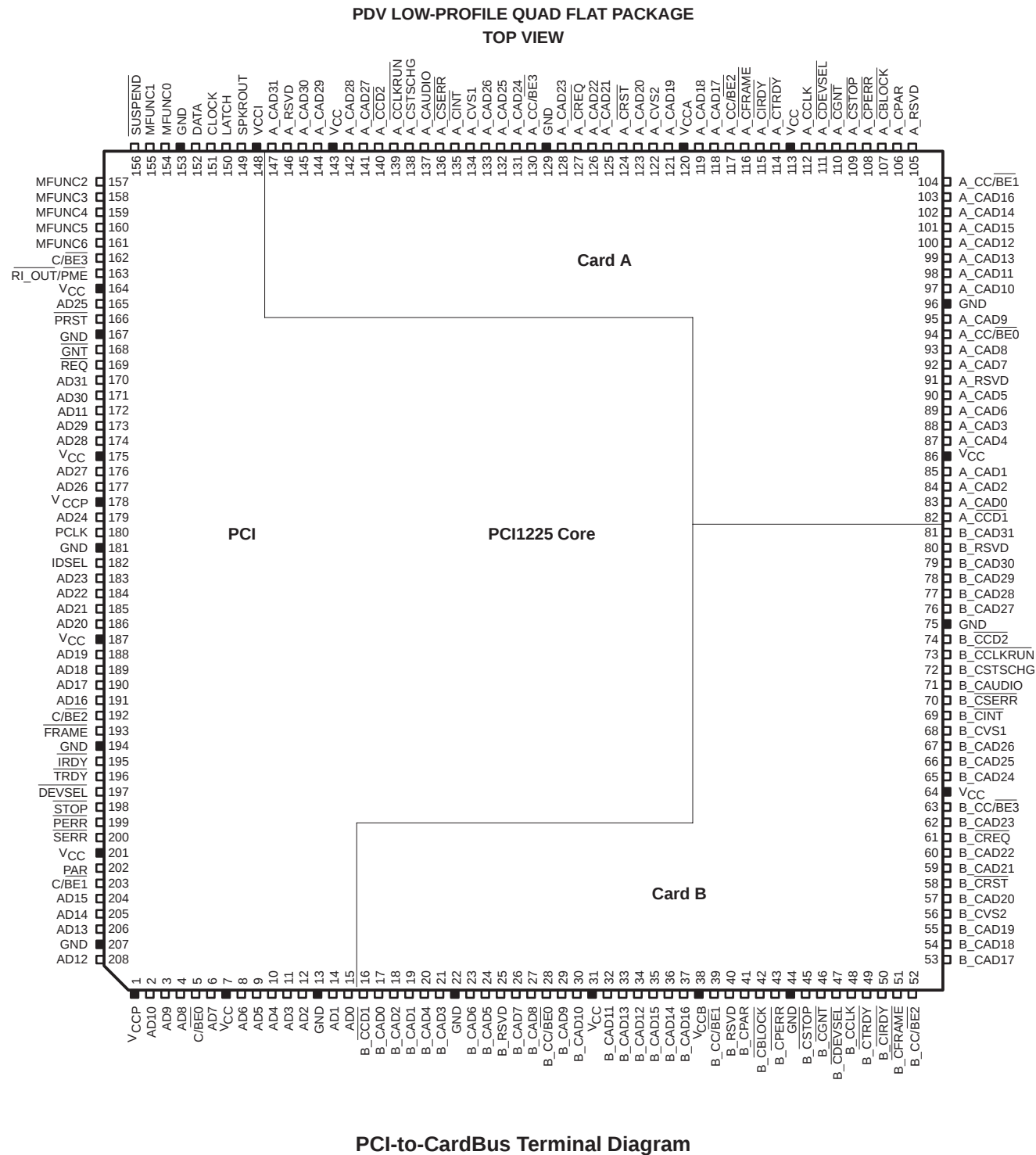
PCI-to-CardBus Terminal Diagram
