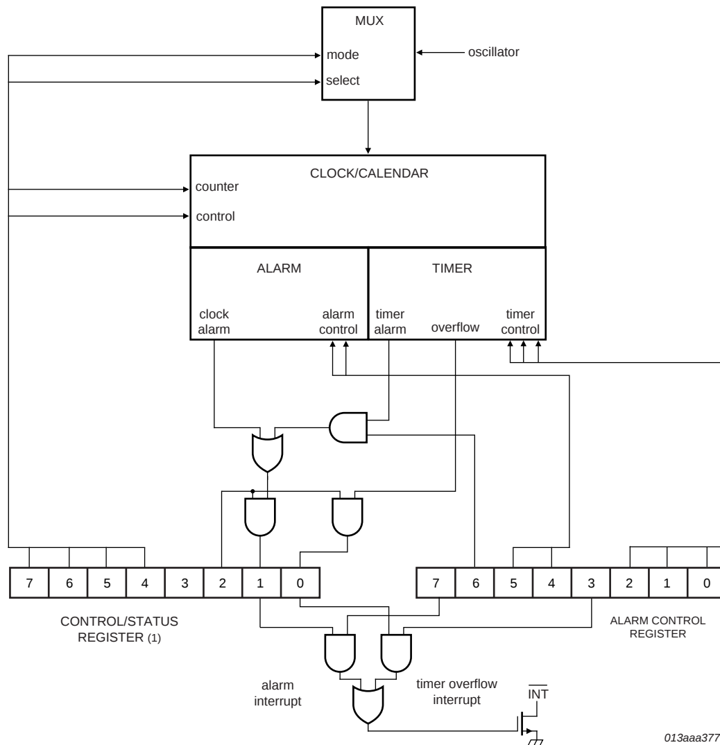
Fig 10. Alarm and timer interrupt logic diagram
