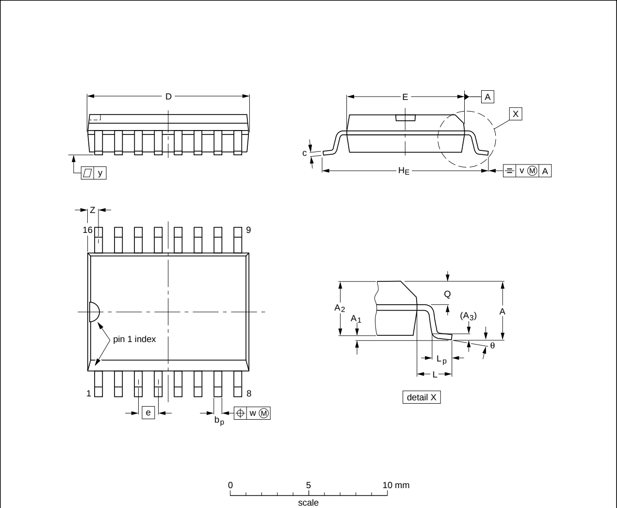
SO16: plastic small outline package; 16 leads; body width 7.5 mm
