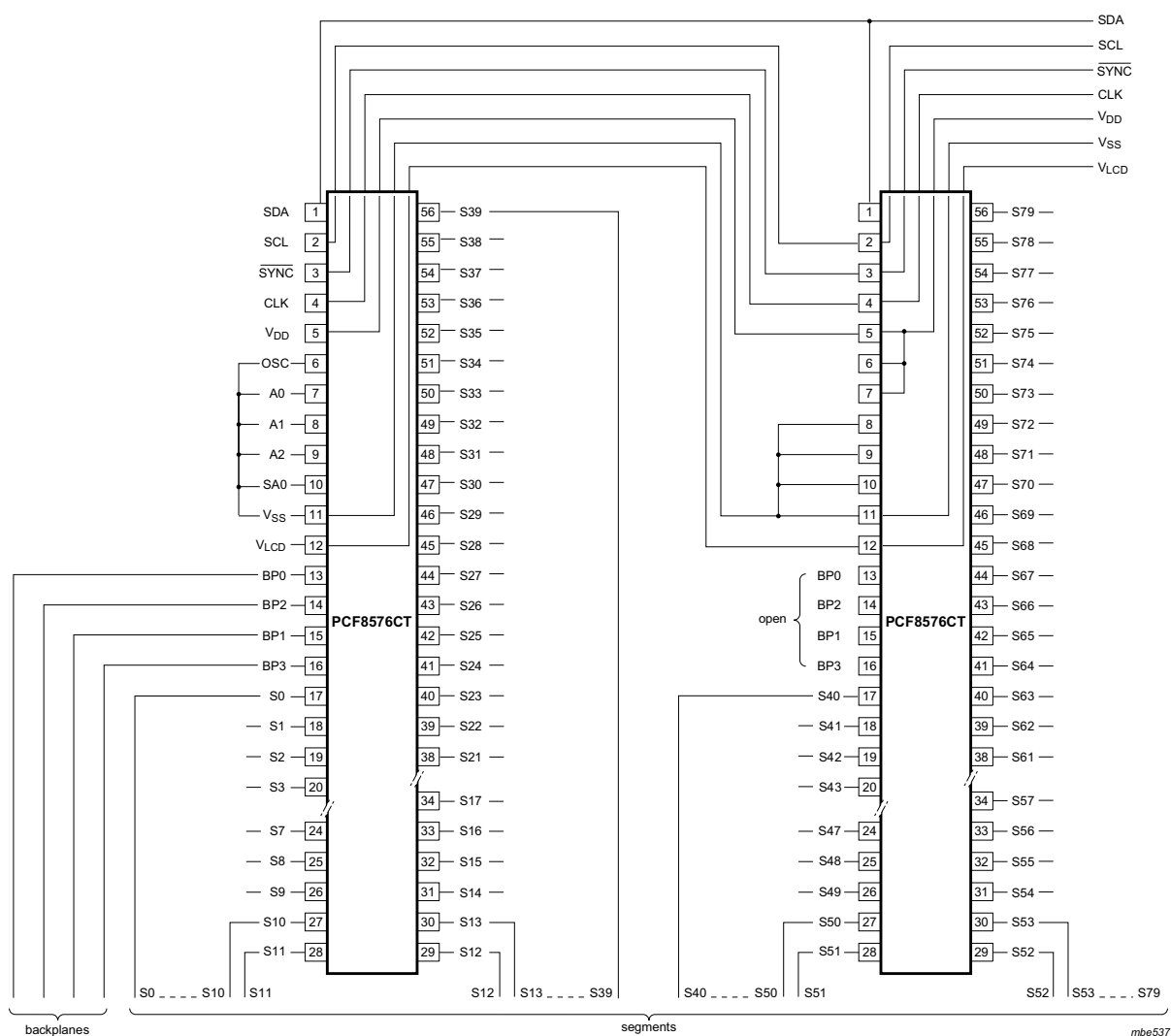
Fig 32. Single plane wiring of packaged PCF8576CT
