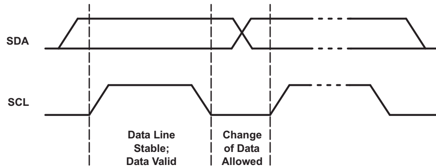
Figure 16. Bit Transfer
