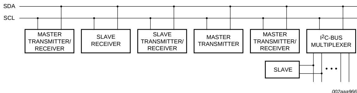
Fig 13. System configuration
