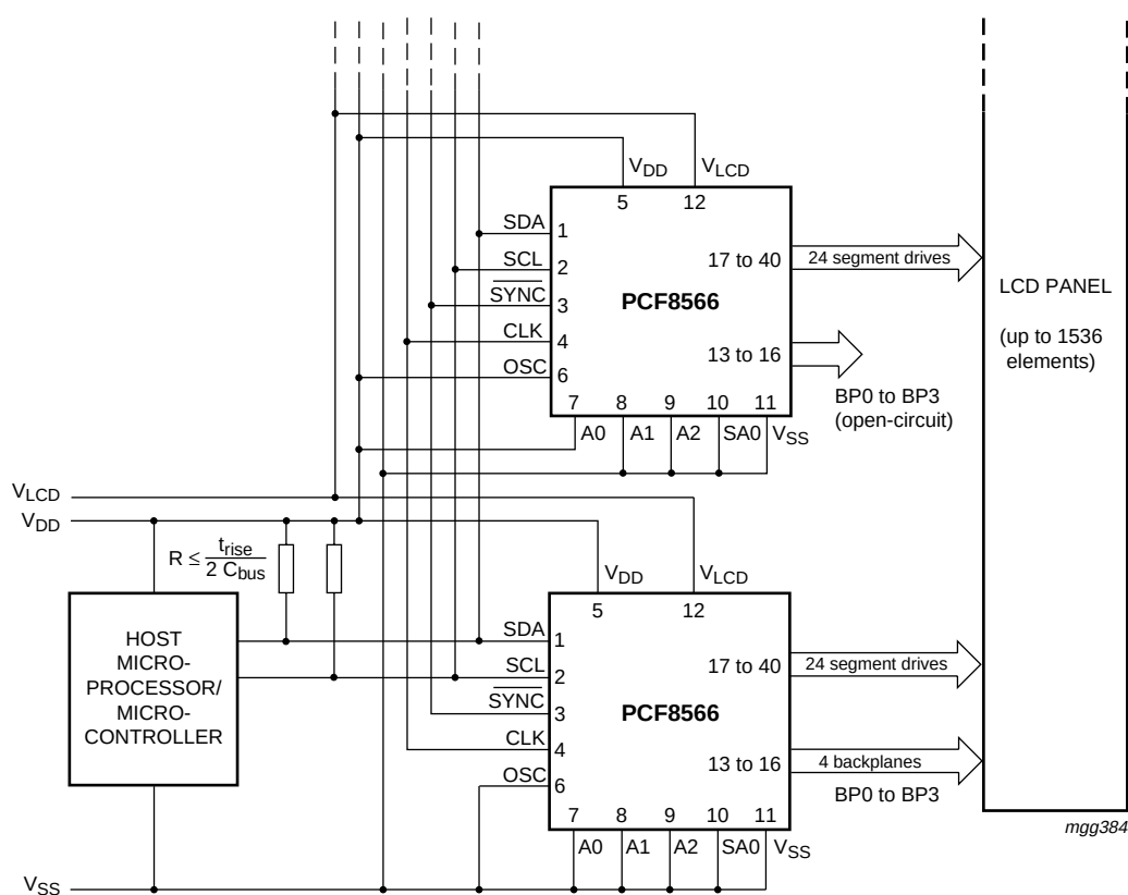
Fig 26. Cascaded PCF8566 configuration
