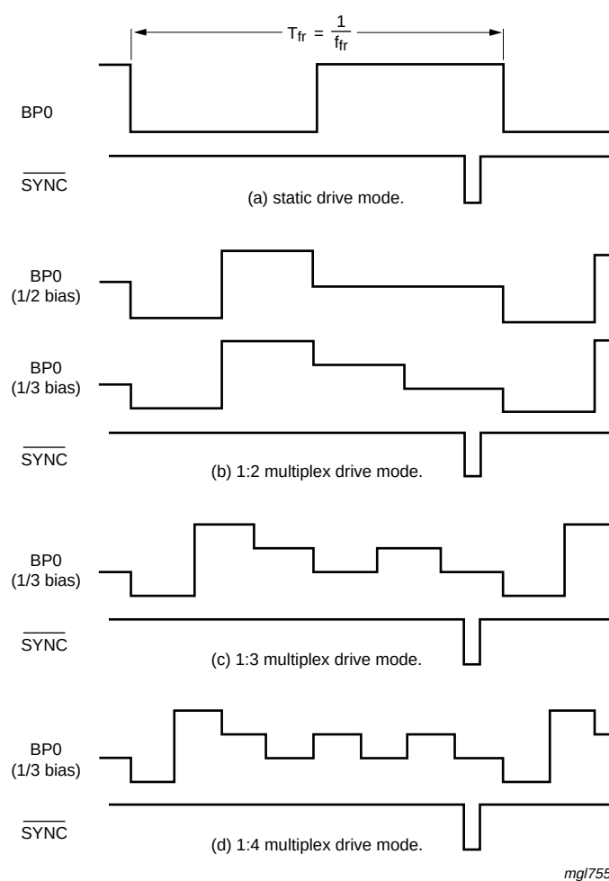
Fig 27. Synchronization of the cascade for the various PCF8566 drive modes
