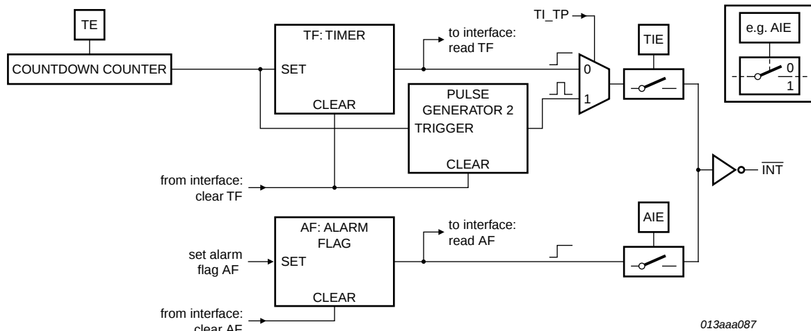
Fig 6. Interrupt scheme
