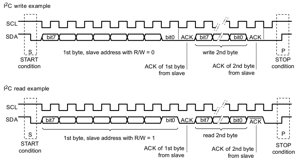
Fig 33. I 2 C read and write signaling
