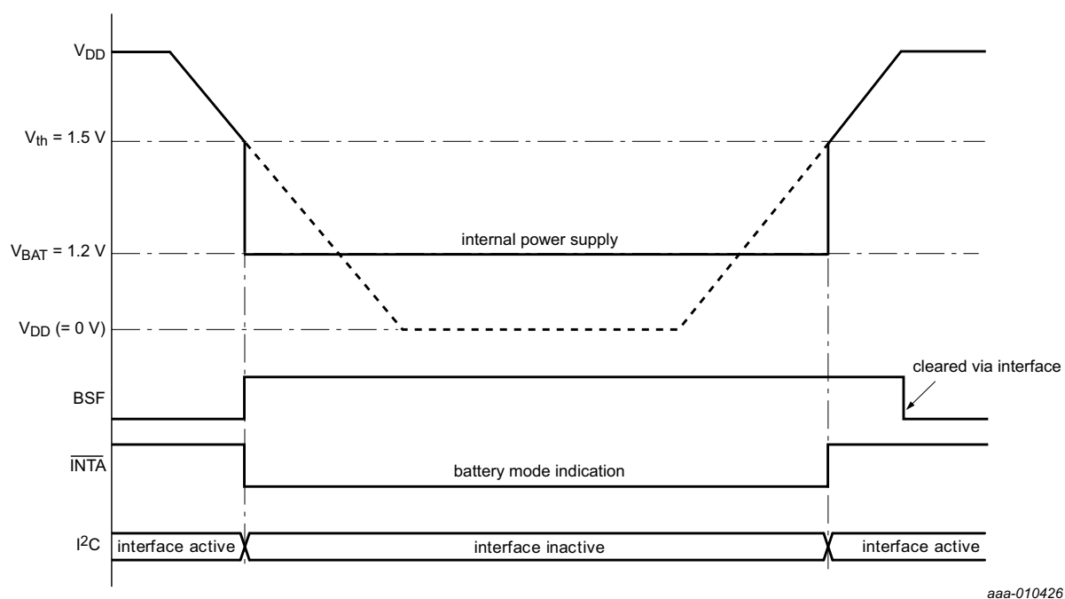
Fig 25. Switching at the higher of V_{BAT} or V_{th}
