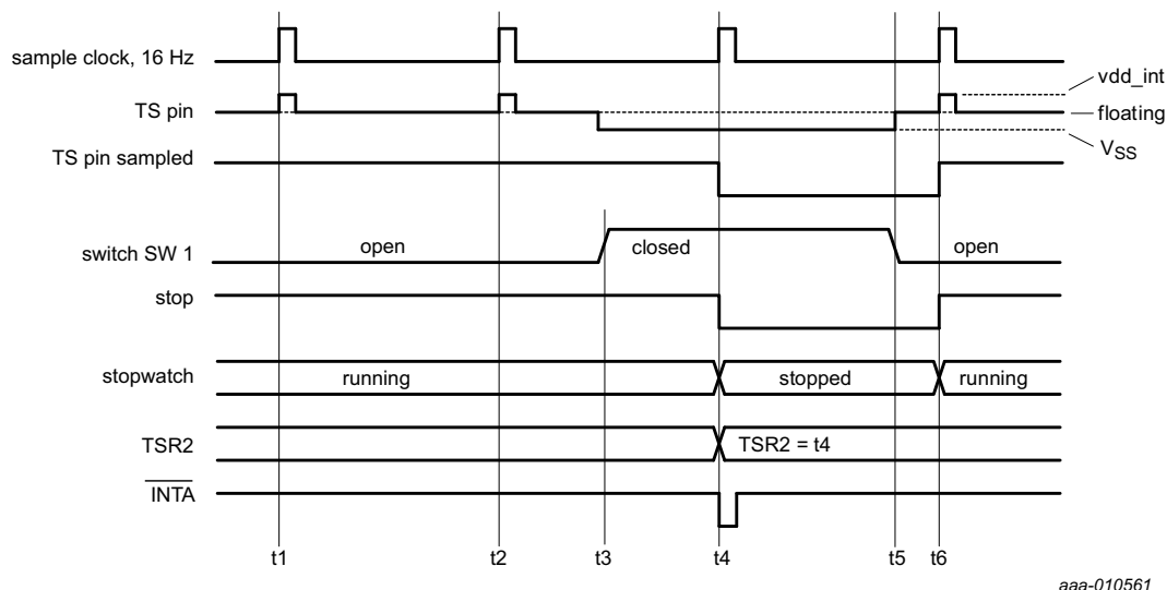
Fig 35. Application example timing
