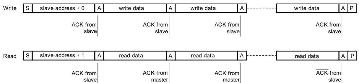
Fig 32. I 2 C read and write protocol
