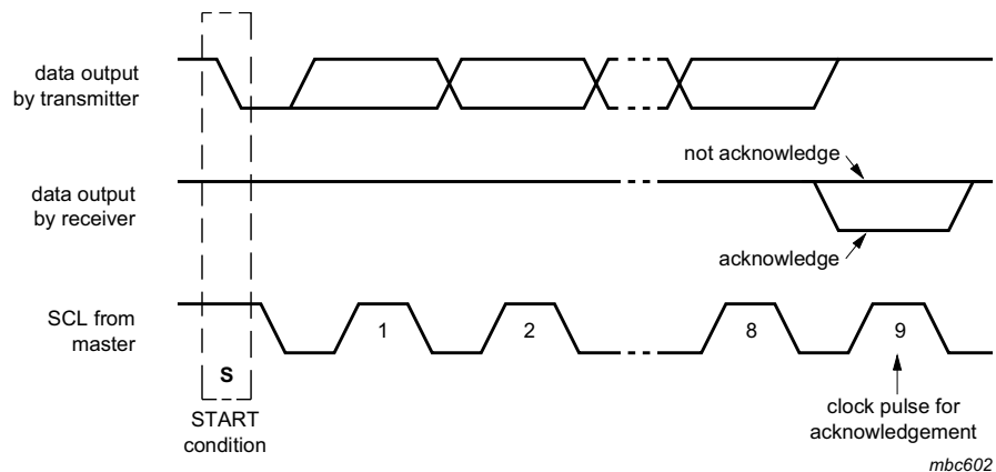
Fig 16. Acknowledgement of the I 2 C-bus
