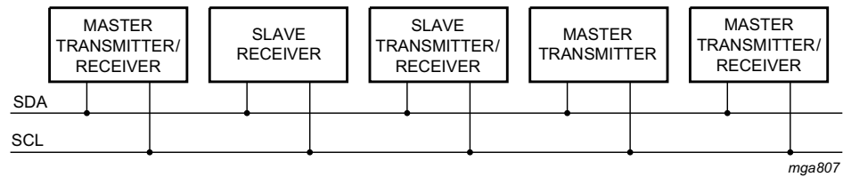
Fig 15. System configuration
