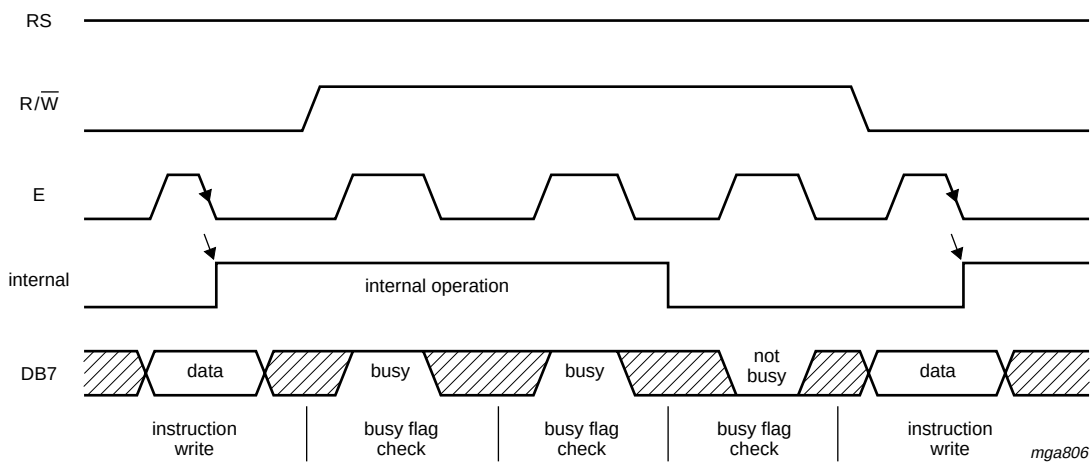
Fig 24. Example of busy flag checking timing sequence
