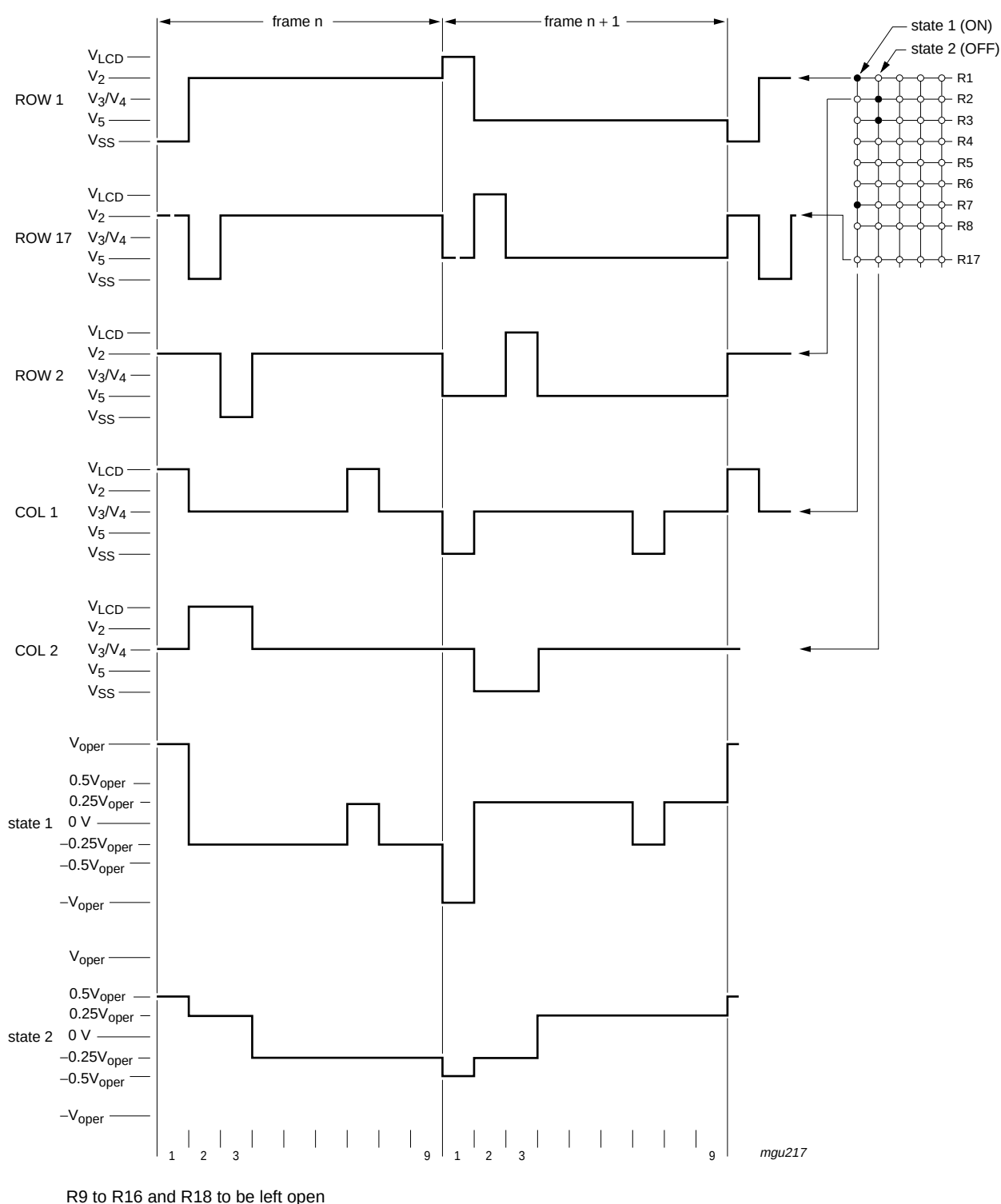
Fig 14. MUX 1:9 LCD waveforms; Character mode
