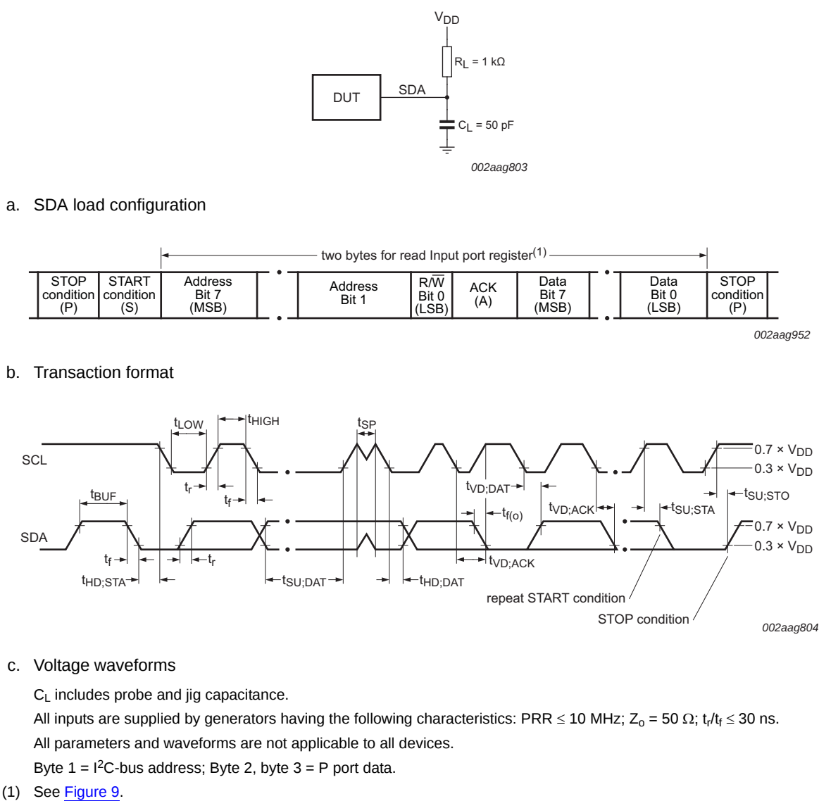
Fig 29. I 2 C-bus interface load circuit and voltage waveforms
