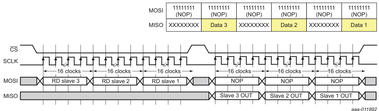
Fig 16. Read access
