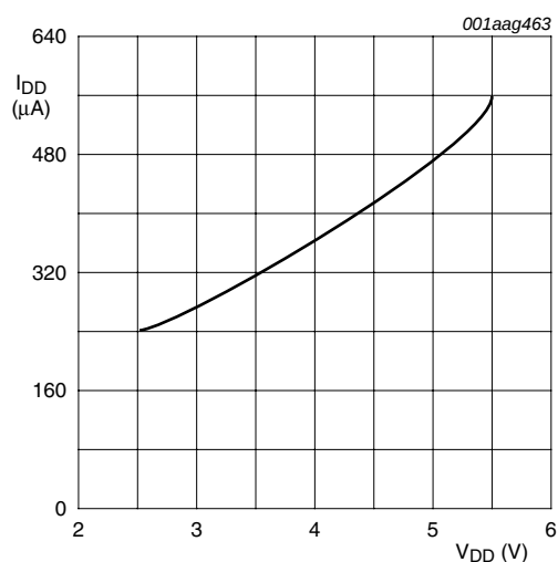
Fig 21. Operating supply current as a function of supply voltage (typical)
