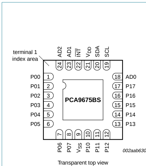
Fig 7. Pin configuration for HVQFN24
