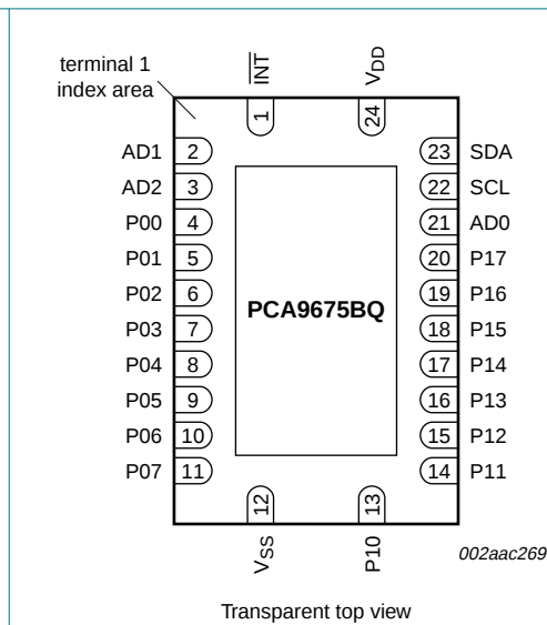
Fig 8. Pin configuration for DHVQFN24
