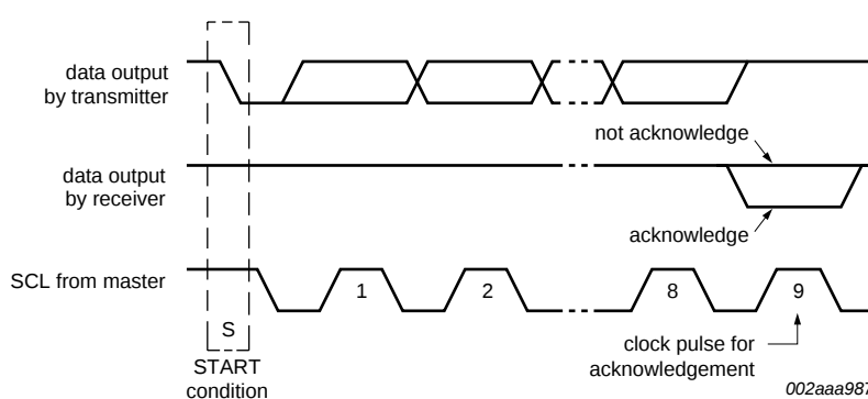
Fig 19. Acknowledgement on the I 2 C-bus
